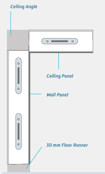
MATRIX 60, 85 and 105 - WITHOUT FLOOR
