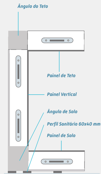
MATRIX 60, 85 e 105 - COM SOLO
