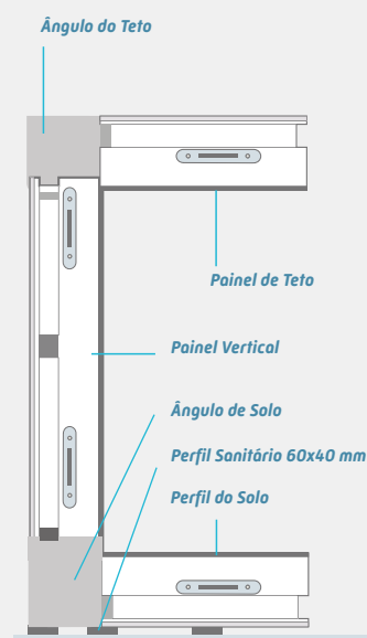
MATRIX 150 - COM SOLO
