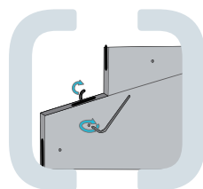
MATRIX 150: 30x10 mm insulation between panels and corners
